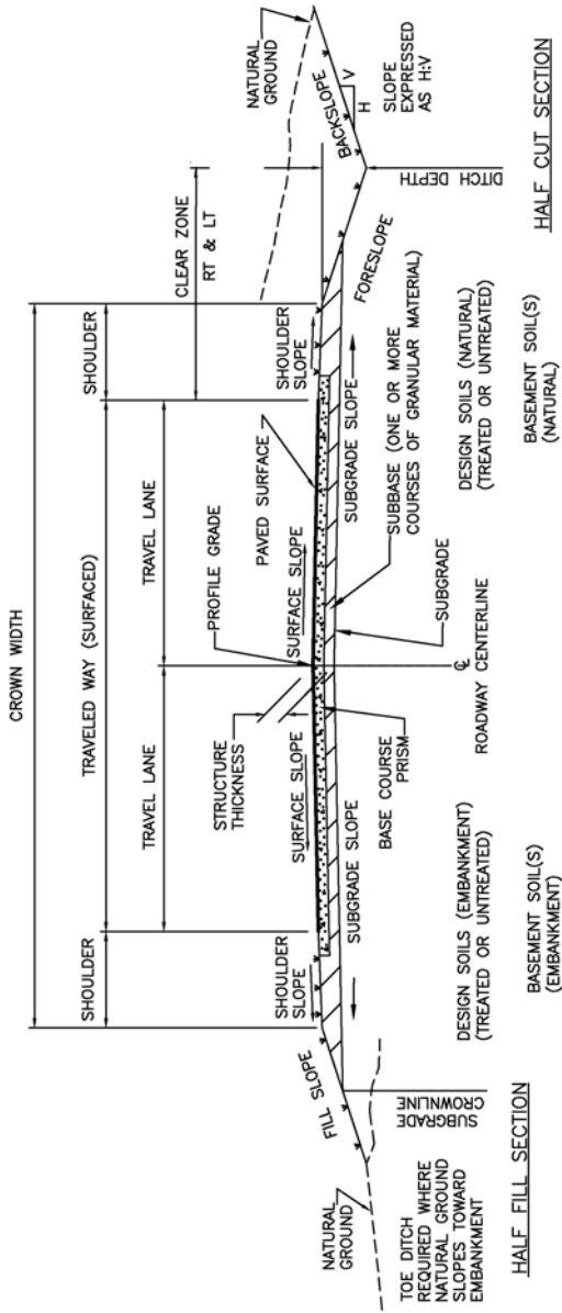
FIGURE — 1. PAVEMENT STRUCTURE (To Subgrade Crownline)
